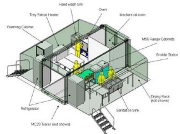
Expeditionary Field Kitchen
